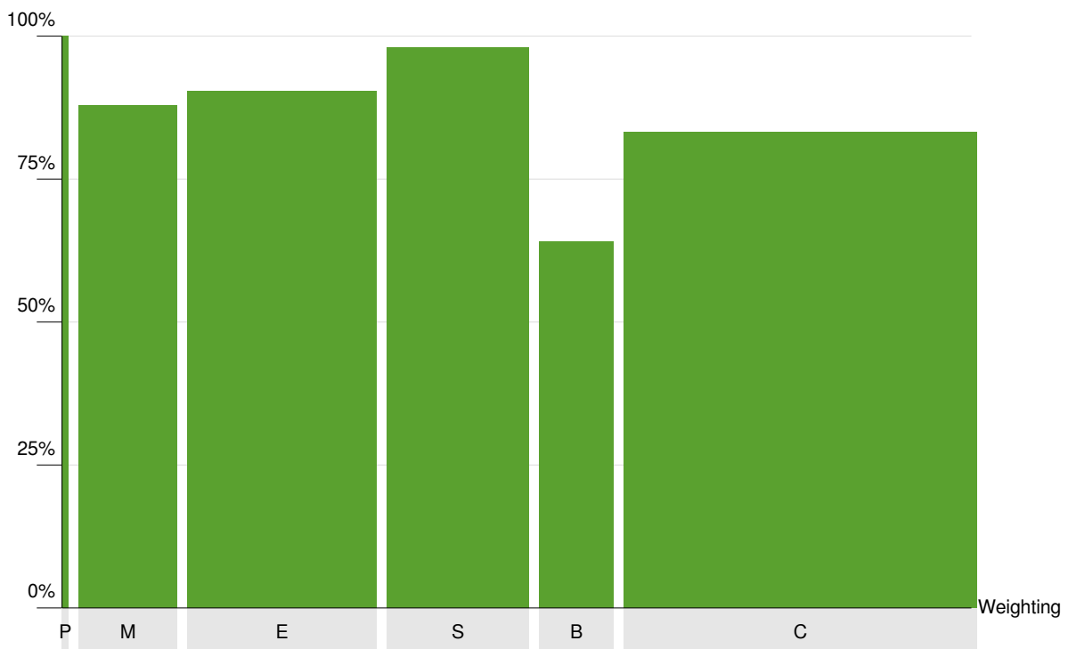
Section scores
